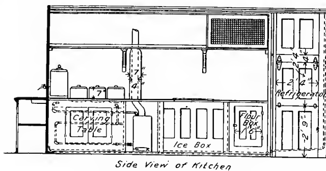
Fig. 476. Side Elevation of Kitchen.
